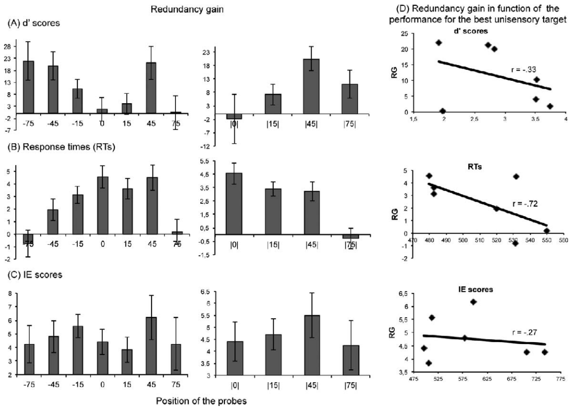
Figure 4. RG (in percent) based on d' scores (A), RTs (B), and IE scores (C) as a function of the eccentricity. (D) RG in function of the performance for the best unisensory component based on d' , RTs, and IE scores. Error bars denote standard errors of the mean corrected for between-subjects variability (Cousineau, 2005).
