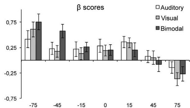
Figure 3. \beta scores for the discrimination of auditory, visual, and audio-visual stimuli as a function of the eccentricity. Positive values reflected a leftward response bias, while negative values represented a rightward response bias. Error bars denote standard errors of the mean corrected for between-subjects variability (Cousineau, 2005).
