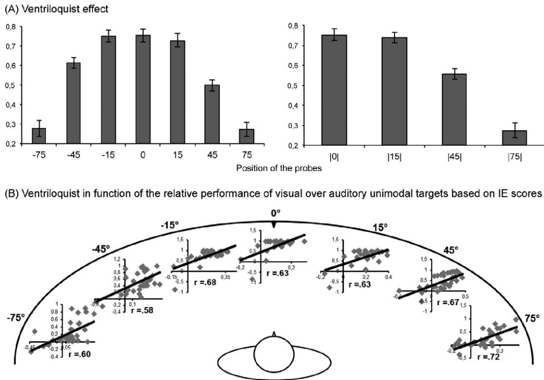
Figure 6. (A) Ventriloquist effect as a function of the eccentricity. This score is obtained by subtracting the percentage of responses guided by hearing to the percentage of responses guided by vision for each eccentricity. Error bars denote standard errors of the mean corrected for between-subjects variability (Cousineau, 2005). (B) Ventriloquist effect as a function of the relative reliability between visual and auditory targets. This figure shows a significant positive correlation between the ventriloquist effect and the visual reliability scores for each eccentricity.
