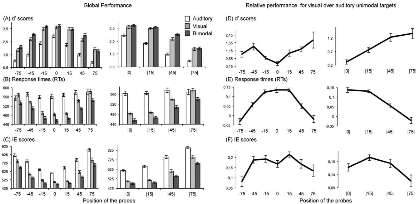
Figure 2. Left panel: d' scores (A), RTs (B), and IE scores (see Methods) (C) for the discrimination of auditory, visual, and audio-visual stimuli as a function of the eccentricity. Right panel: relative performance for visual over auditory targets as a function of the eccentricity based on d' scores (D), RTs (E), and IE scores (F). Error bars denote standard errors of the mean corrected for between-subjects variability (Cousineau, 2005).
