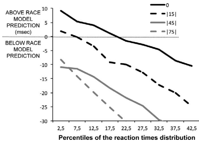
Figure 5. Race model inequality. Test for violation of the race model inequality (Miller, 1982; Ulrich, Miller, & Schröter, 2007). The graph represents the difference in milliseconds (on the y-axis) between the model prediction computed from the RTs of each unisensory counterpart (the model bound) and the RTs obtained in the redundant conditions. Positive values on the graph refer to RTs that were faster than the race model prediction. Negative values on the graph refer to RTs that were slower than the race model prediction. The difference between the bound and the RTs of the redundant condition are computed for each percentile of the RT distribution (on the x-axis).
